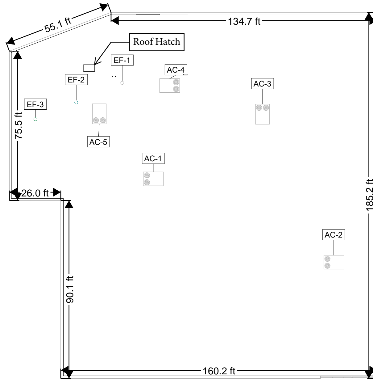
① ROOF PLAN 1" = 30'-0"
